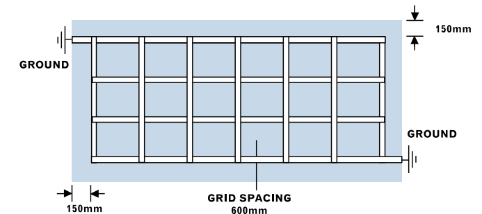
Figure 7.2 Earth strip layout
