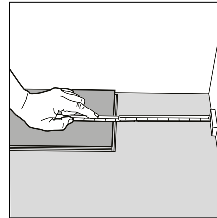
Figure 6.13 Last plank, first row
