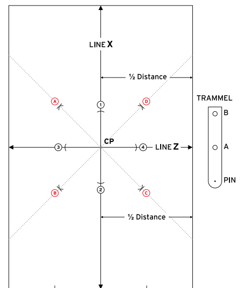
Figure 6.7 Marking out diagonal tiling
