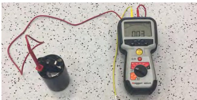
Figure 7.3 Test electrode
